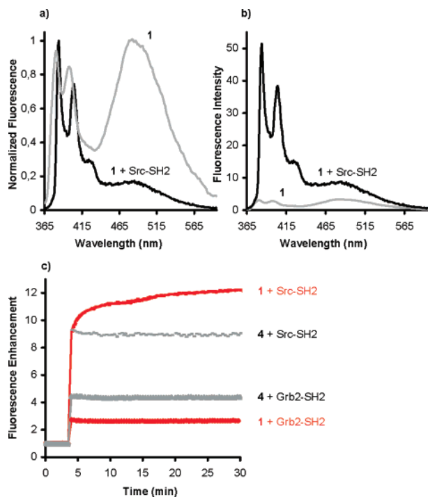
Figure 2. Fluorescence of HPB 1 and PB 4 : (a) normalized fluorescence spectra of 1 before (gray) and after addition of Src-SH2 (black); (b) fluorescence spectra of 1 before (gray) and after addition of Src-SH2 (black line); (c) time course of relative fluorescence intensity at 380 nm of 1 (red) or 4 (black) after addition (5 min) of Src-SH2 and Grb2-SH2. Conditions: \lambda_{\text{ex}} = 340 nm, 1 \mu\text{M} of 1 in buffer (20 mM \text{NaH}_2\text{PO}_4 , 100 mM NaCl, 2 mM DTT, pH 7.4, 25 °C) and 16 \mu\text{M} SH2 protein (required for saturation of signaling) when added.
